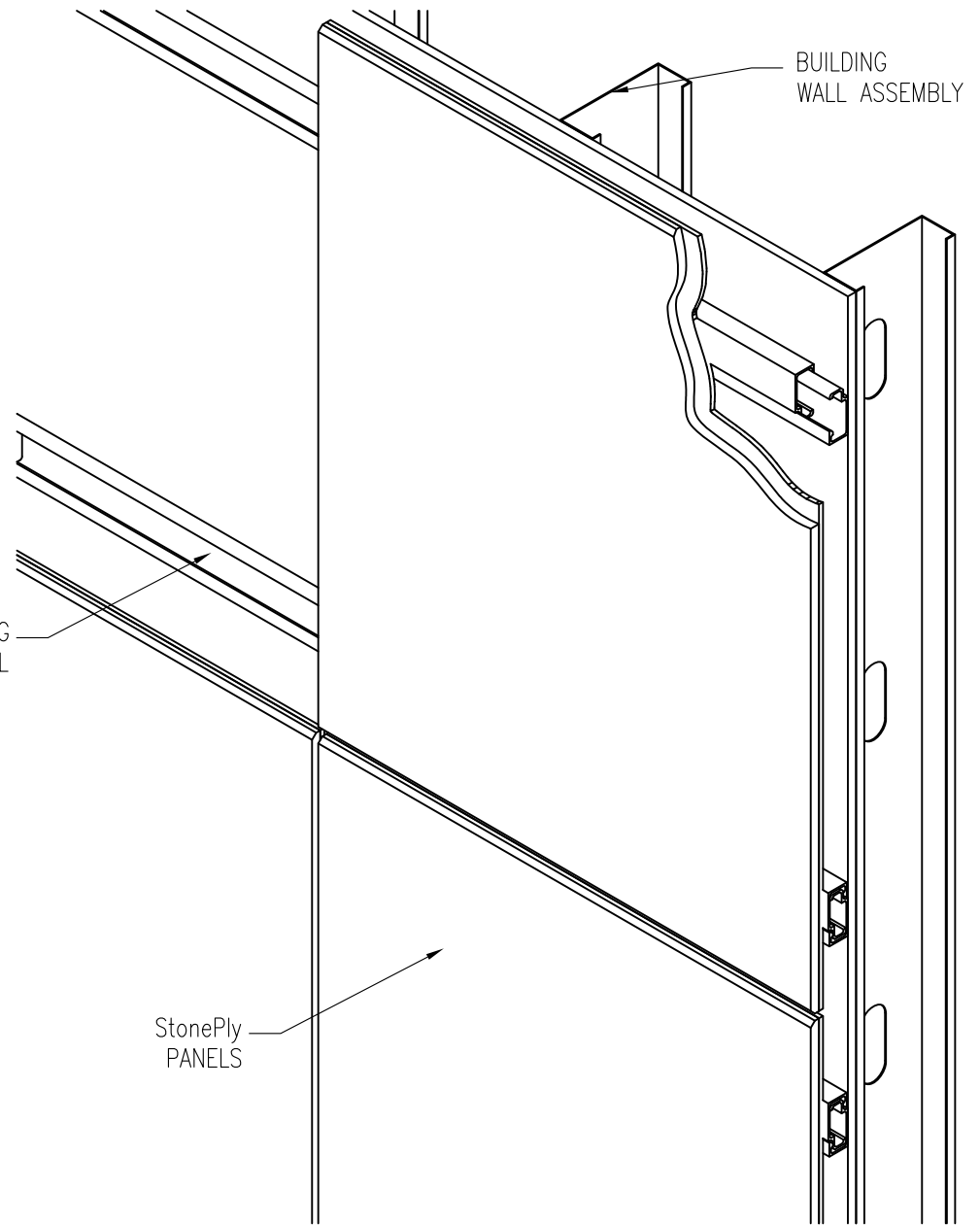
D1 INTERLOCKING PANELS NTS
